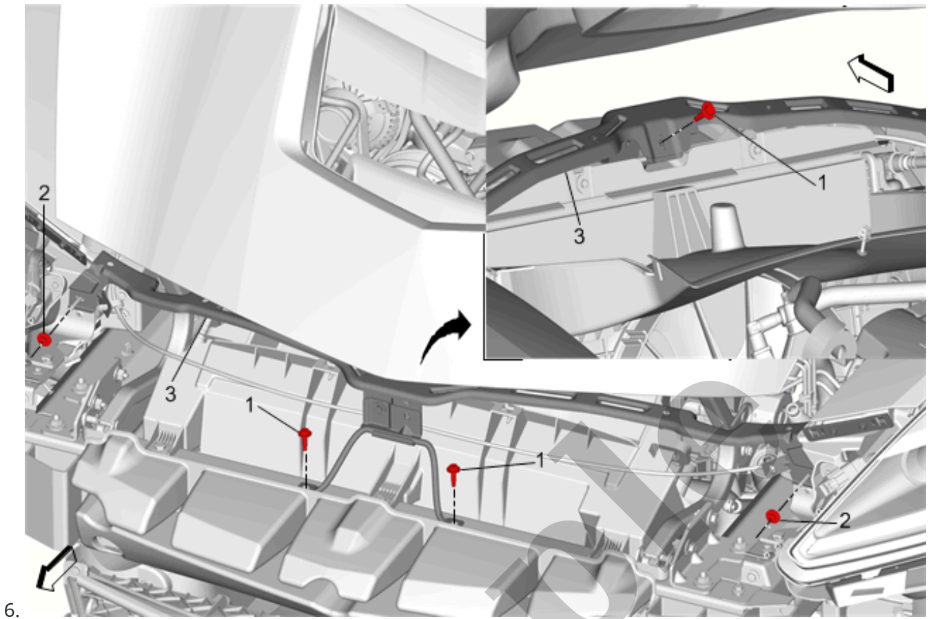
6. Front Bumper Fascia Center Support Replacement (2)@Charge Air Cooler Radiator »Install
